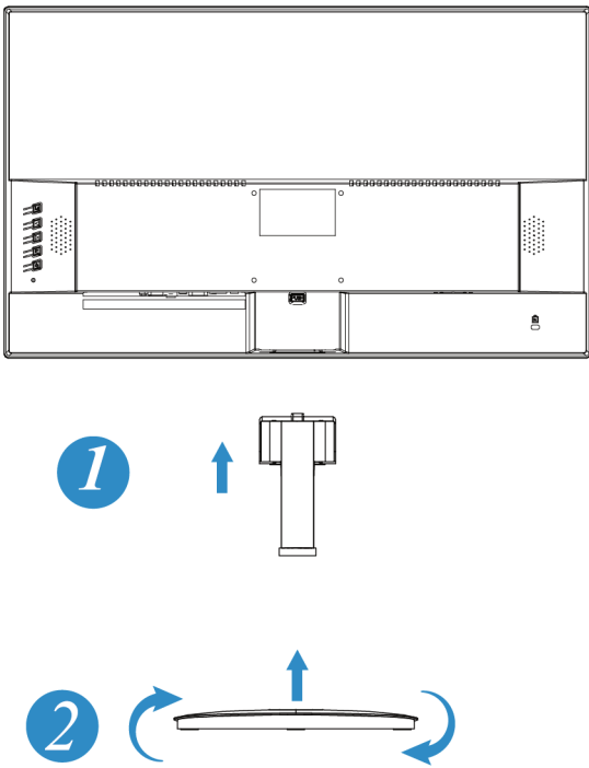
Figure.1. Installing and Removing the Base
